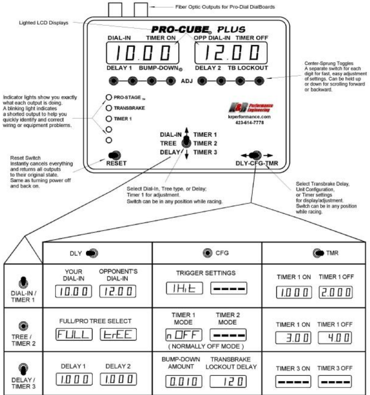
FACTORY DEFAULT SETTINGS FOR MODEL PCT1-P ARE SHOWN IN THIS TABLE (SEE "TIMER OUTPUT CONFIGURATION" SECTION FOR MODEL PCT1-P)
